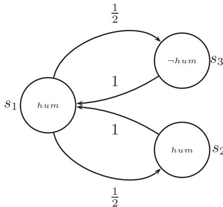
FIG. 2. A model satisfying \Gamma , assuming the nephew has \frac{1}{2} probability of failing to return the ball.
